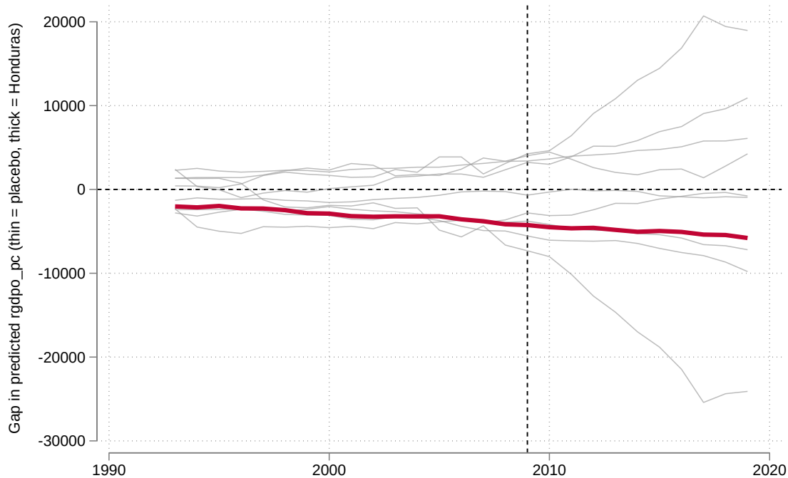
Central America & the Caribbean: factors_yrs (outliers excluded)
